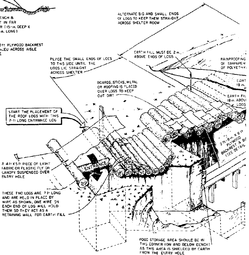
Fig. A-2.1. Log-Covered Trench Shelter, Pictorial View
